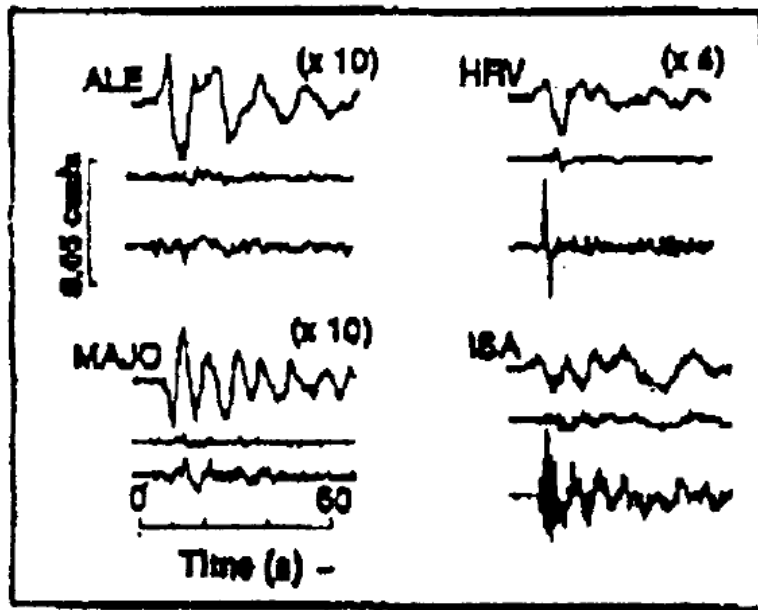
Fig. 4. Broad-band velocity records from four stations (ALE: epicentral distance A = 5185 km azimuth = 9 : HRV: A = 4366 km, azimuth = 69 , MAJO: A = 8029 km azimuth - 306 , ISA: A = 745 km azimuth = 132 ) for the main shock (top trace) and the first (middle) and second (lower) aftershocks. The amplitudes of the seismograms at ALE, HRV and MAJO are increased relative to ISA for display. The large amplitudes of the second aftershock relative to the other two events in the long-strike azimuth (ISA) is attributable to rupture directivity.
