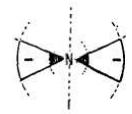
Fig. 28 Curvature increases as potentials divide and multiply
