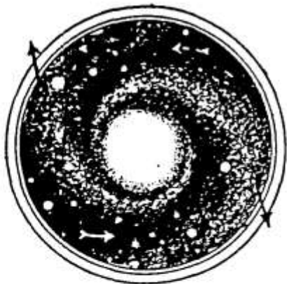
Fig. 35 Light comes from darkness and darkness from light
