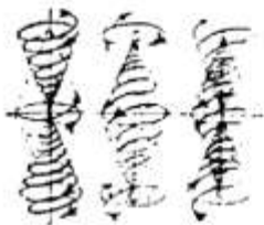
Fig. 52 Atomic systems forming
