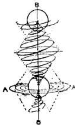
Fig. 53 AA Atomic systems forming BB Wave shaft
