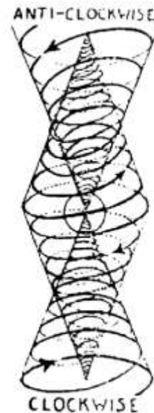
Fig. 60 Direction of spiral motion never reverses
