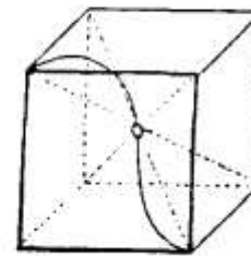
Fig. 47 The six outer mirrors of gravitation
