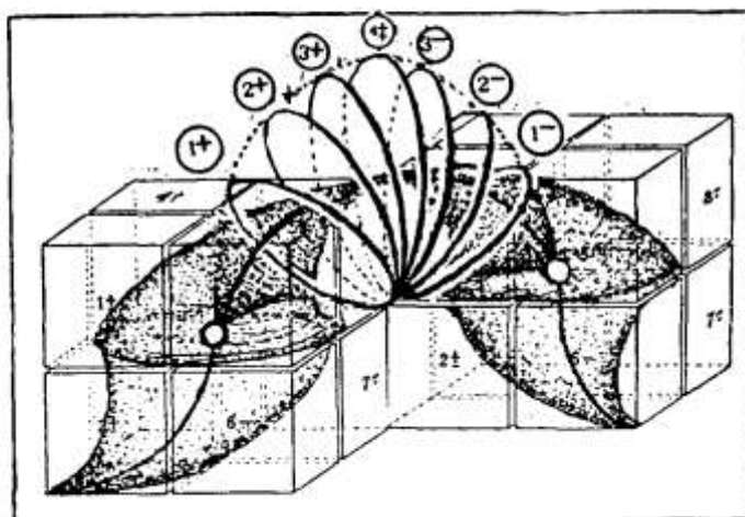
Fig. 76 The octave gyrosopic principle
