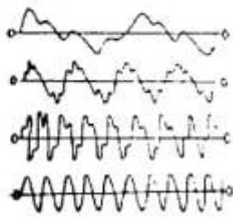
Fig. 59 Various patterns of wave shafts recording borrowed energy
