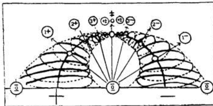
Fig. 73 Cycle of the elements from rest to rest
