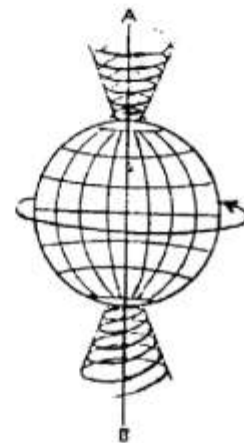
Fig. 55 AB—The shaft of earth and moon
