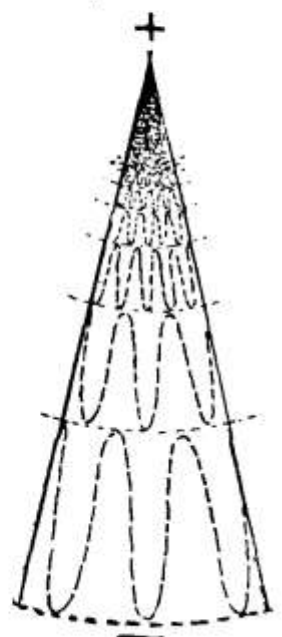
Fig. 31 The division and multiplication principle
