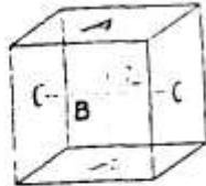
Fig. 40 The six wave field boundary planes
