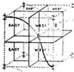
Fig. 48 The six inner micro-radiation
