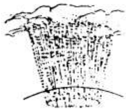
Fig. 45 Rain falling vertically forms cone
