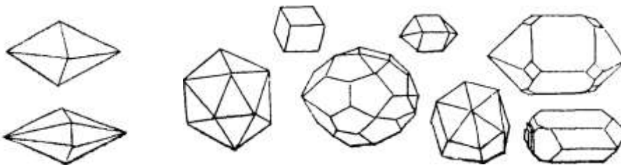
Fig. 15 All crystals are cube sections
