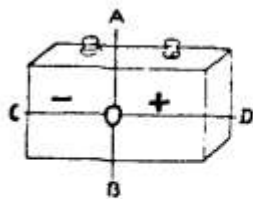
Fig. 20 Balanced interchange between equal conditions
