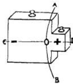
Fig. 22 Interchange between unequal opposites
