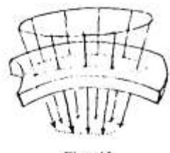
Fig. 43 Light rays are radial when projected through spherical planes
