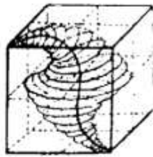
Fig. 49 Wave spirals on the wave shaft
