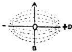
Fig. 21 Symmetry of the cube AB Static equator CD Dynamic equator
